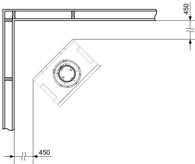
ME stove with side glass
