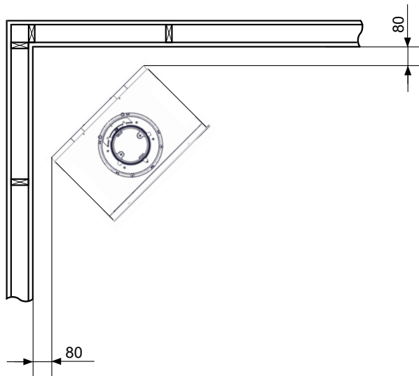
ME stove without side glass
