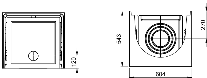
Capri High extension part
