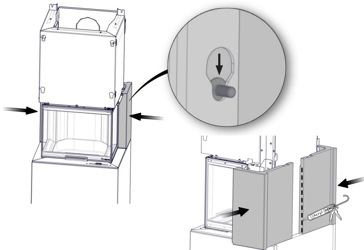
FIG 13 b Capri High_Q-24UL
