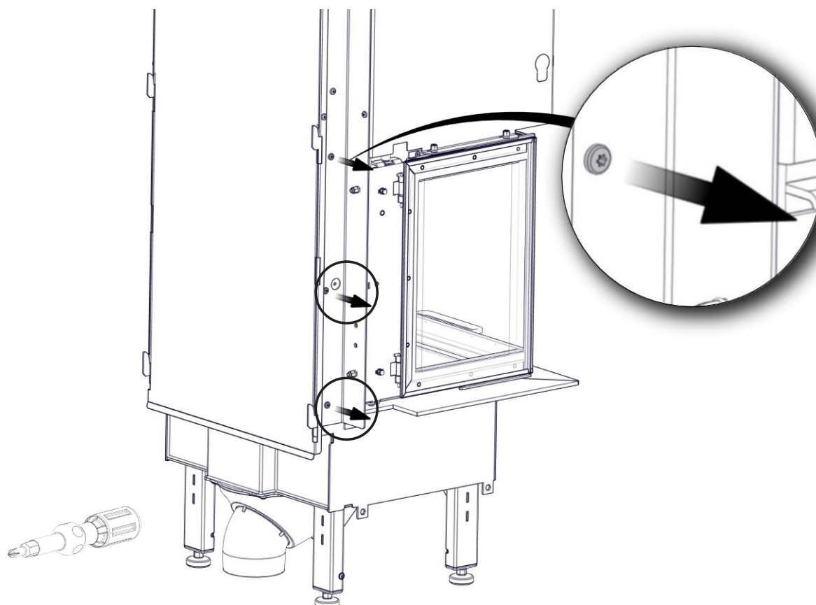
FIG 8 b Capri High_Q-24UL
